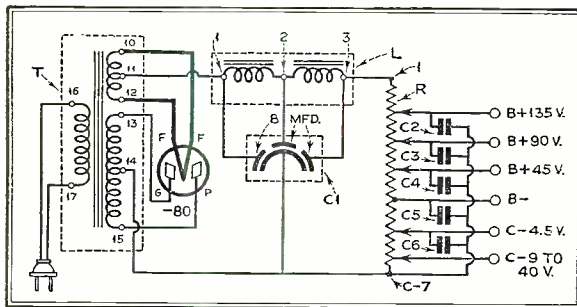
This is the schematic circuit of the B and C power supply. It jibes completely with the picture diagram above. The dotted lines indicate those units which are self contained, such as T, the transformer; L, the filter choke, etc.
