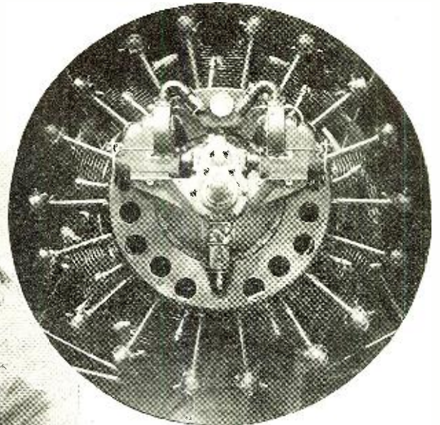
(Above) Shielding applied to an airplane engine in order to suppress interference, thereby making radio reception possible
