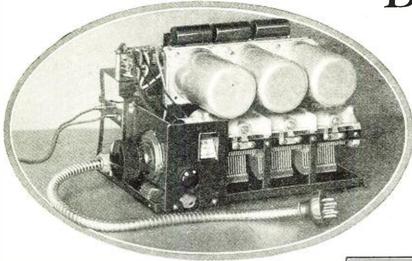
Compactness is the order of the day in the design of auto-radio receivers. Above, the front view of the National job. Note the absence of remote tuning controls, tuning being accomplished by a vernier knob, as in any other type of radio receiver
