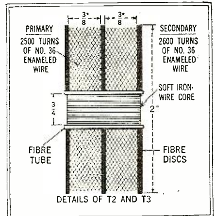
Fig. 3. Cross section view of an intermediate frequency transformer
