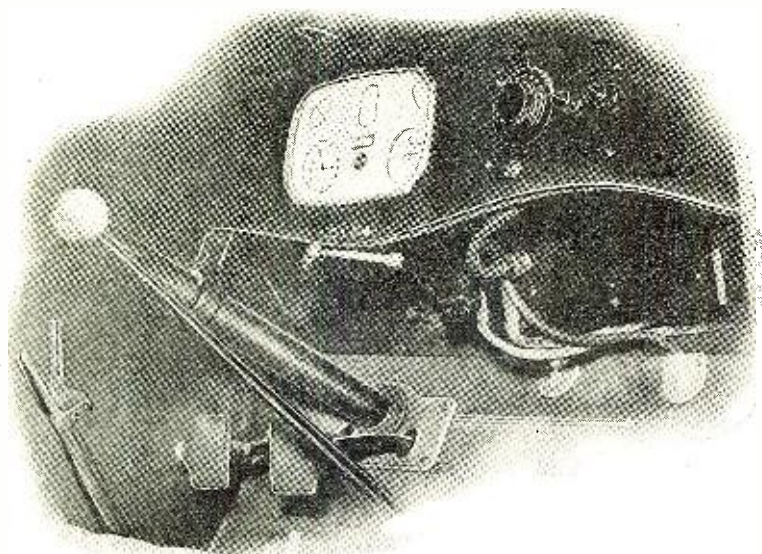
Tuning controls mounted on the dash operate the compactly built receiver conveniently located near the floor of the car
