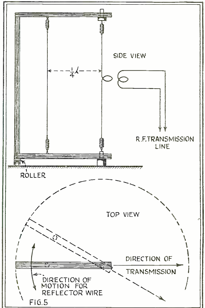
Fig. 5—A practical directional antenna. A single reflector wire is pivoted so that it can be rotated around the transmitting aerial for directional transmission or reception
