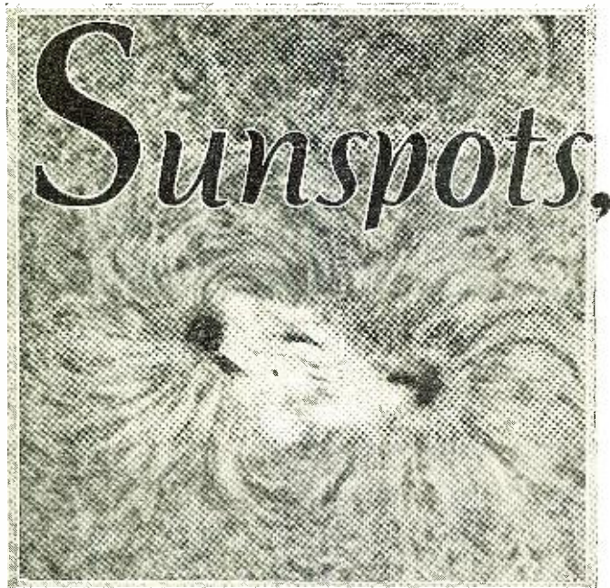
Mt. Wilson spectroheliograph of hydrogen whirls around a bipolar sunspot group. This photograph was taken in light of a single wavelength, and shows that the spots are in reality gigantic tornadoes
