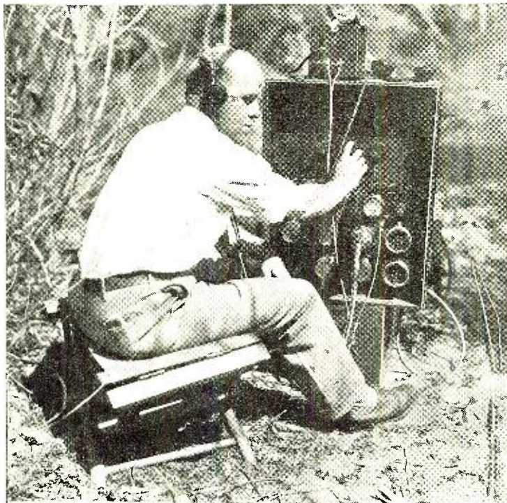
Field mixing panel where the pick-up from the various "mikes" is adjusted to the proper level before being passed along to the recording equipment housed in the truck. The voice signals from planes flying overhead are added to the ground noise before being fed into the recorder
