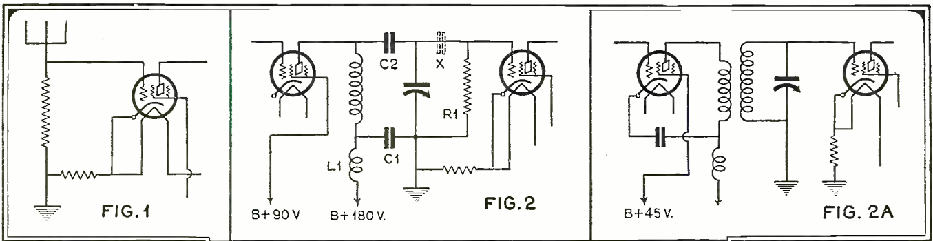
Fig. 1, circuit for coupling antenna to first r.f. stage. Fig. 2, impedance coupling circuit between r.f. stages, illustrating method of isolating plate potential from tuning condenser. Fig. 2A, a standard transformer-coupled r.f. circuit, finally employed
