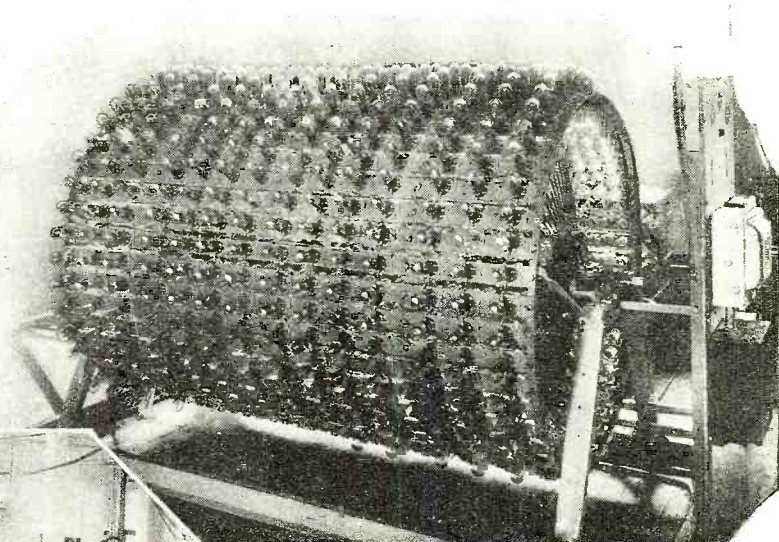
Above: A novel rotary machine, having a capacity of 600 tubes, in which the filaments are put through a process of activation. Left: Assembly tables in the factory. The highest order of precision is called for in the process of manufacture.
