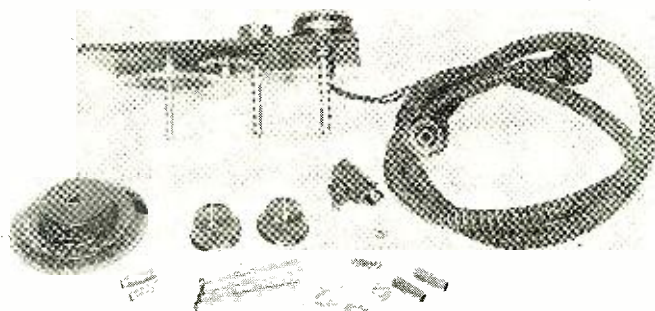
Below are shown the knock-down remote tuning and volume control mechanism and the flexible coupling shaft
