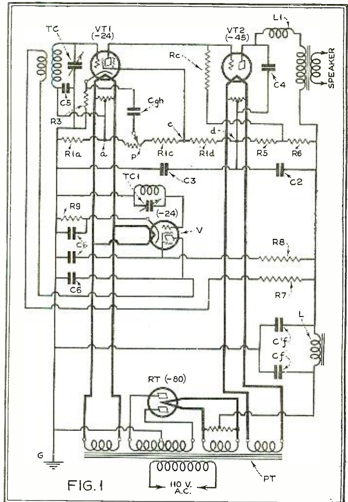
One method of adding two stages of radio frequency amplification to the Loftin-White system
