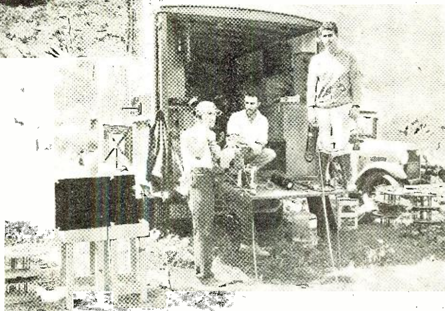
Field mixing panel where the pick-up from the various "mikes" is adjusted to the proper level before being passed along to the recording equipment housed in the truck. The voice signals from planes flying overhead are added to the ground noise before being fed into the recorder
