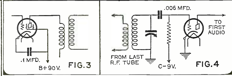
Fig. 3—The transformer-coupled r.f. circuit, employing only by-pass condensers in the screen-grid circuits. Sufficient stability was obtained to make unnecessary the inclusion of r.f. chokes. Fig. 4—Circuit details of the power detector stage
