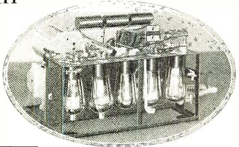
A rear view of the National receiver. Above the tube rack is placed the complete audio resistance-coupled channel of the receiver. Here's a set for car, boat or plane
