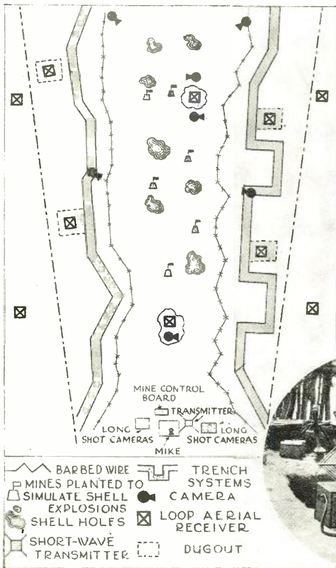
How portable radio receivers are distributed to control movements of large groups in a battle scene. The insert shows a dugout with camera and portable radio receiver used in the filming of a scene from "Flight"
