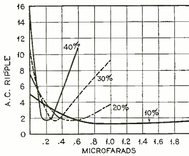
Fig. 5—Ripple measurement curves made with circuit shown in Fig. 4. The ordinates are arbitrary measures of ripple and the abscissæ are variable condenser capacities
